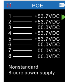
8-core power supply, 53.7V
