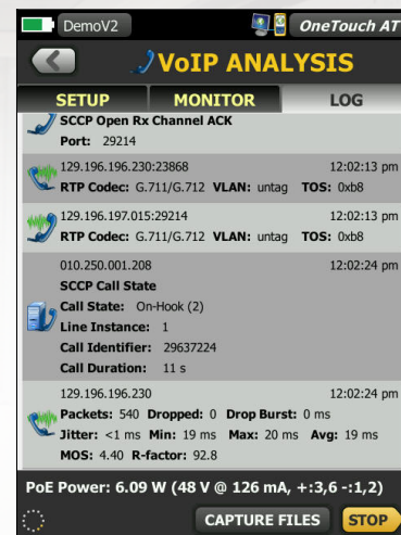
Figure 9. Inline VoIP analysis simplifies troubleshooting of desktop VoIP problems in real-time without TAPs or switch mirror ports
